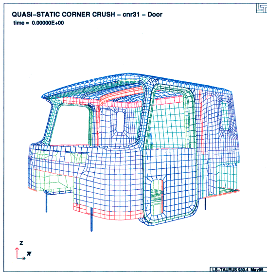
Figure 1 Finite Element mesh of cab.
