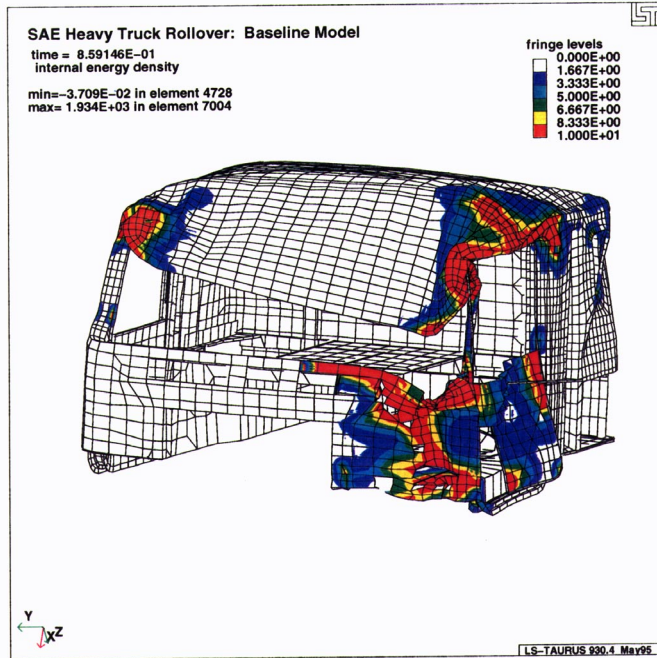
Figure 3 Deformed mesh at 0.86s showing strain energy distributions, localized element failures, and failures of seam welds.
