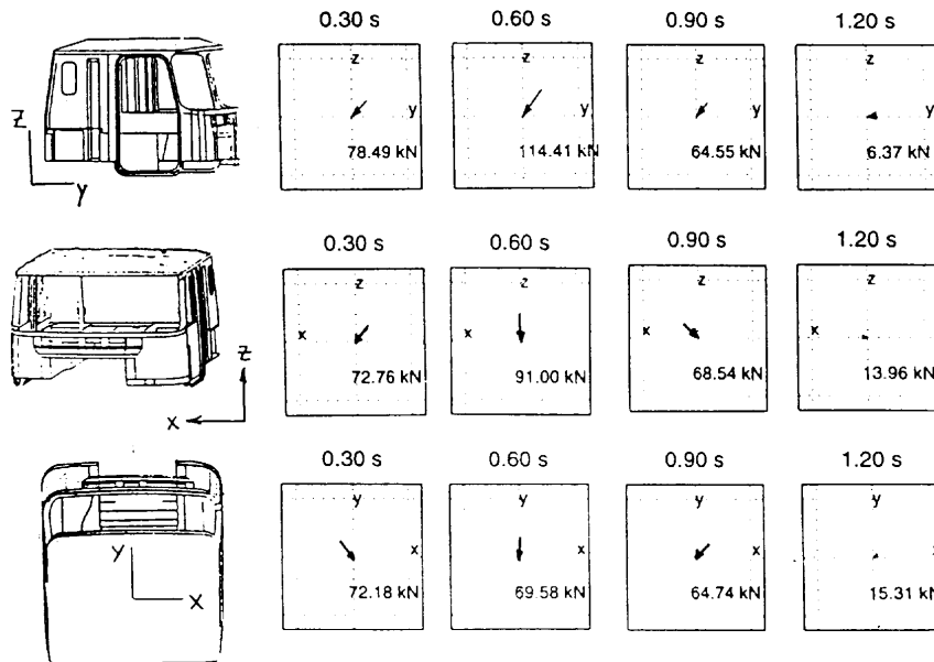
Figure 4 Each row shows the projection of overall ground-to-cab contact force onto one of the cab local coordinate system planes. The magnitudes are the vector resultant of components lying in that plane.
