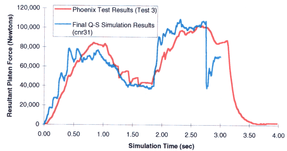
Figure 2 Platen force resultant vs. time.
